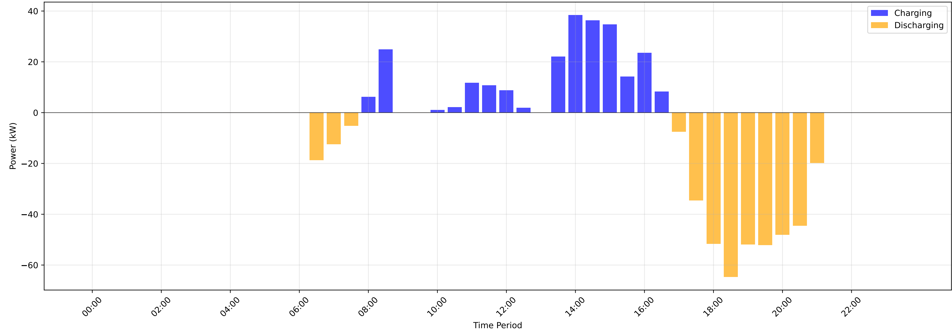
Battery Charge/Discharge Schedule
